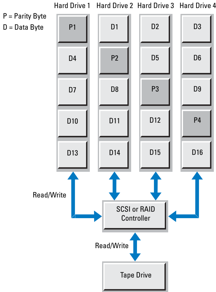
Figure 1-4. Example RAID 5 Configuration
